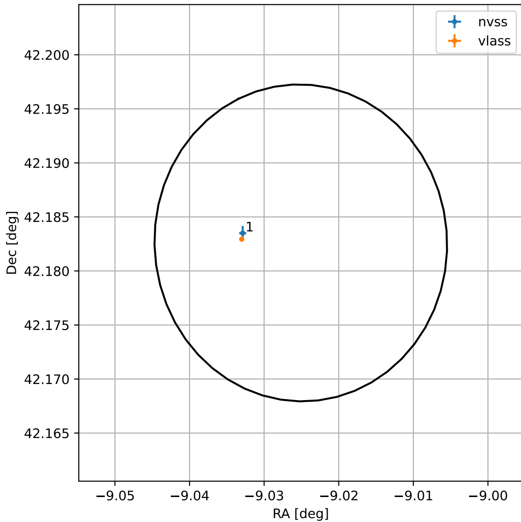
4FGL J2323.8+4210
