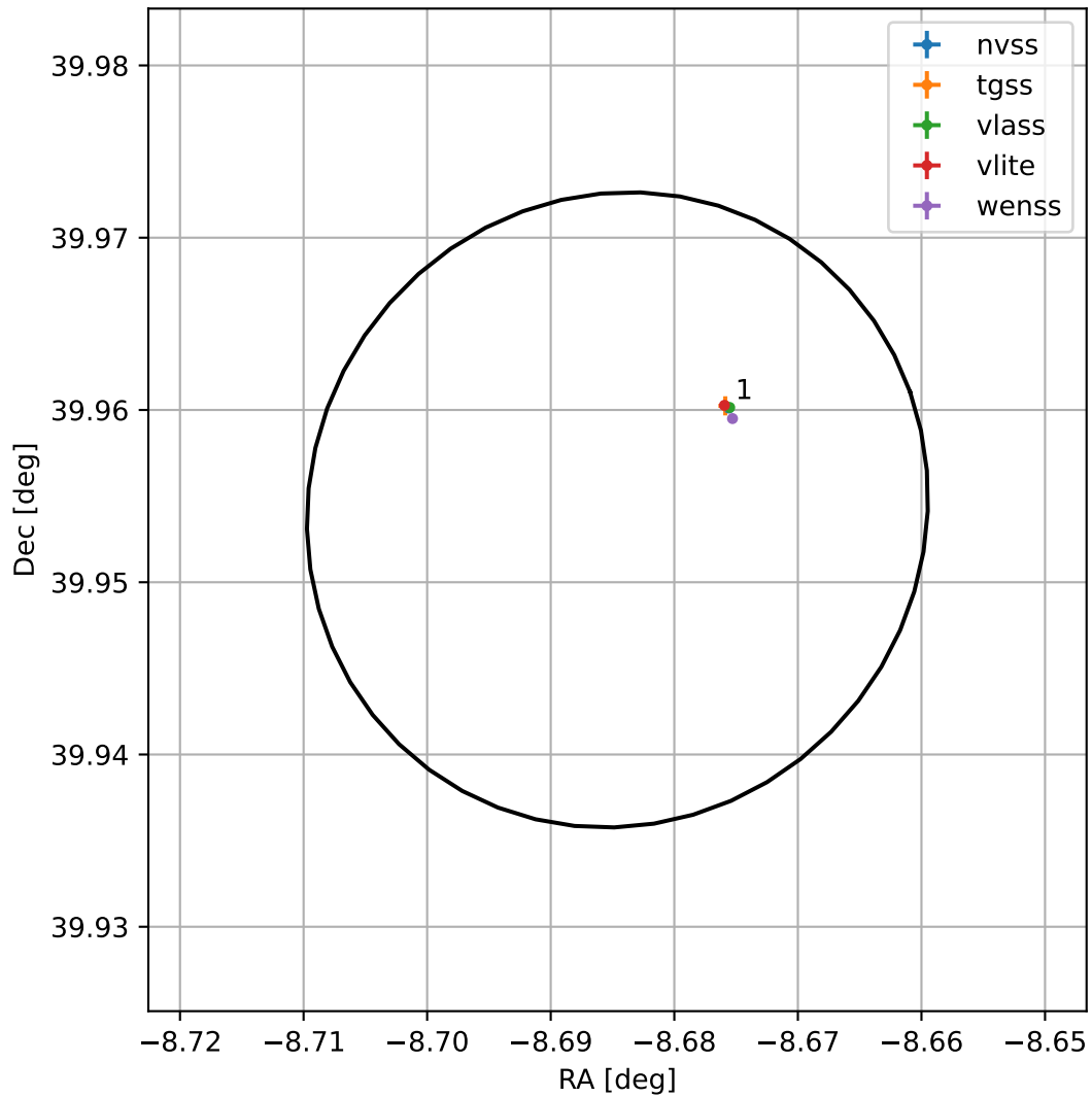
4FGL J2325.2+3957
