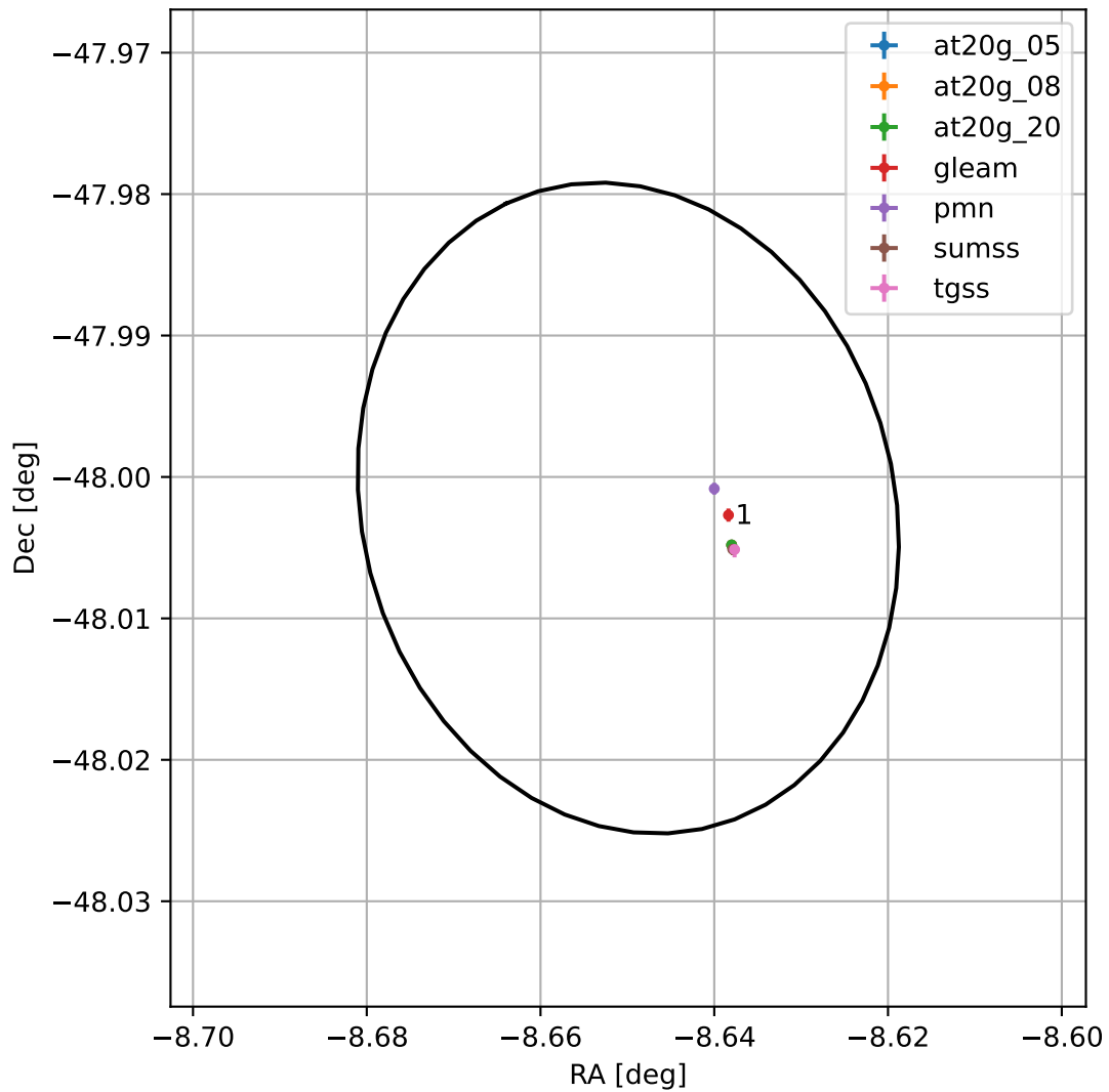
4FGL J2325.4-4800
