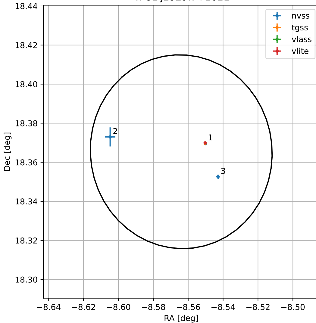
4FGL J2325.7+1821
