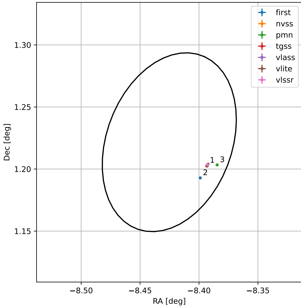
4FGL J2326.2+0113
