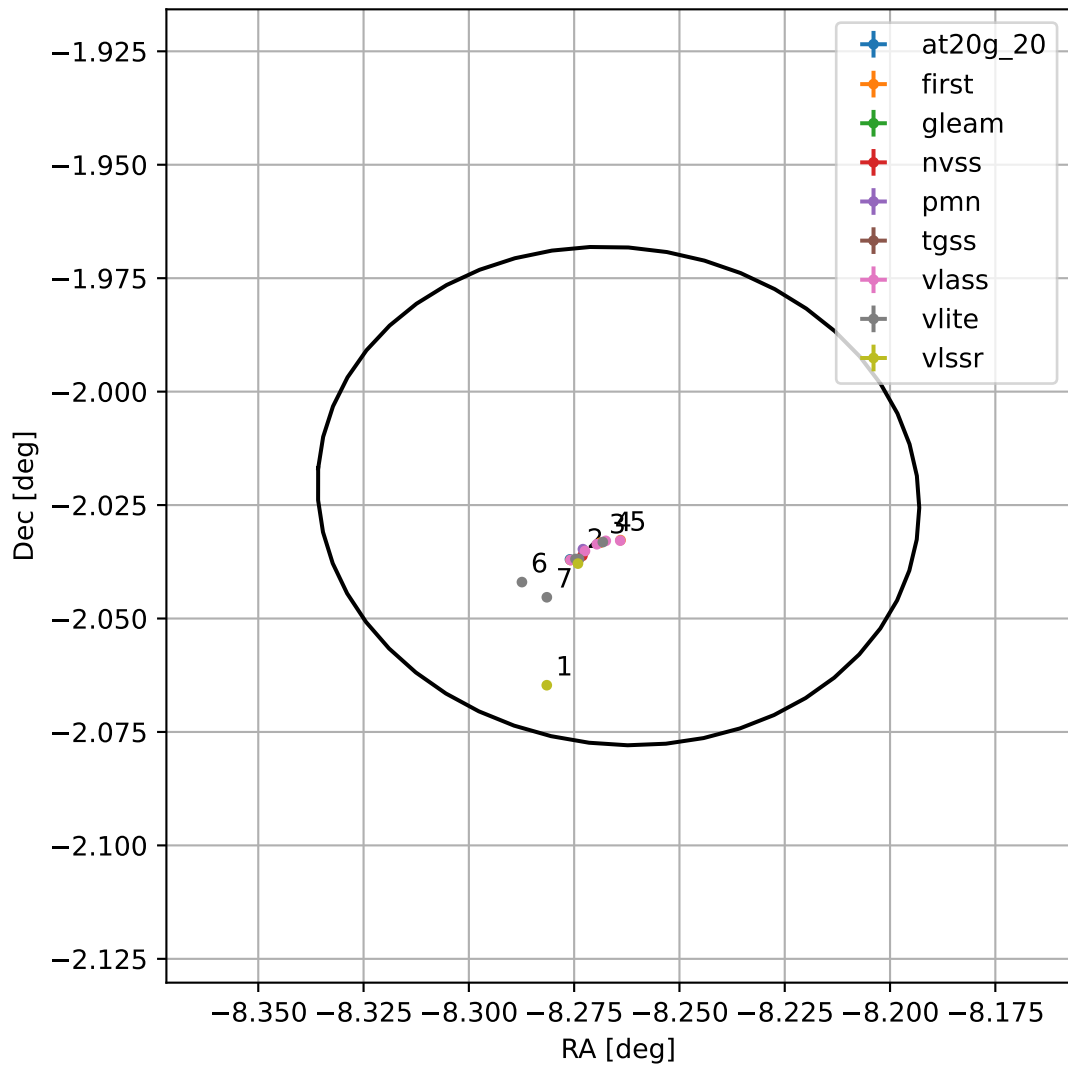
4FGL J2326.9-0201
