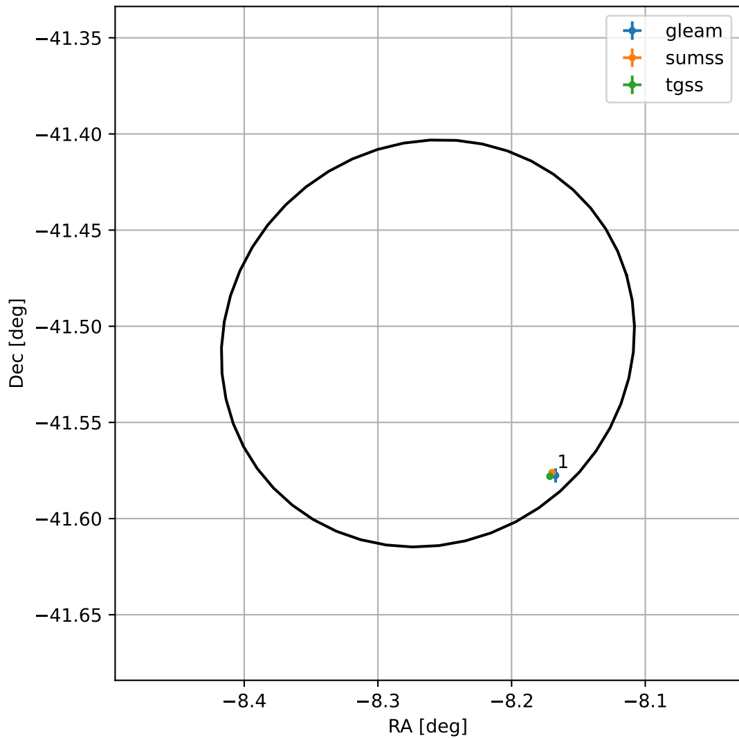
4FGL J2326.9-4130
