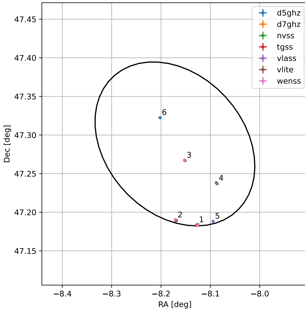
4FGL J2327.3+4717
