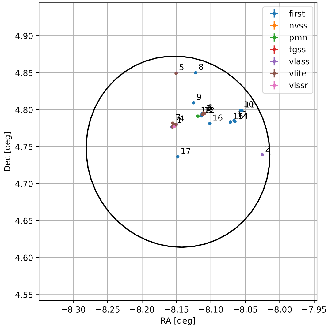
4FGL J2327.4+0444
