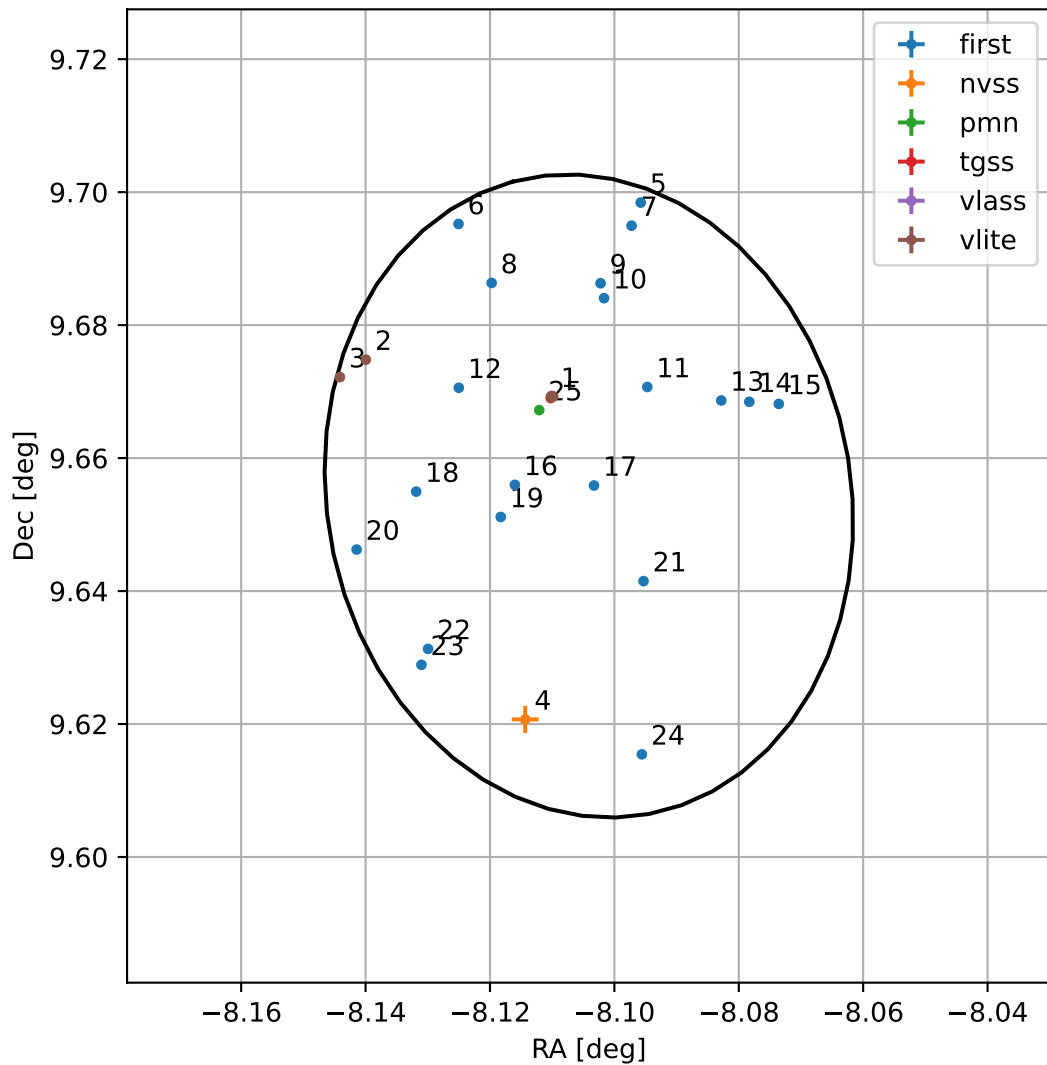
4FGL J2327.5+0939
