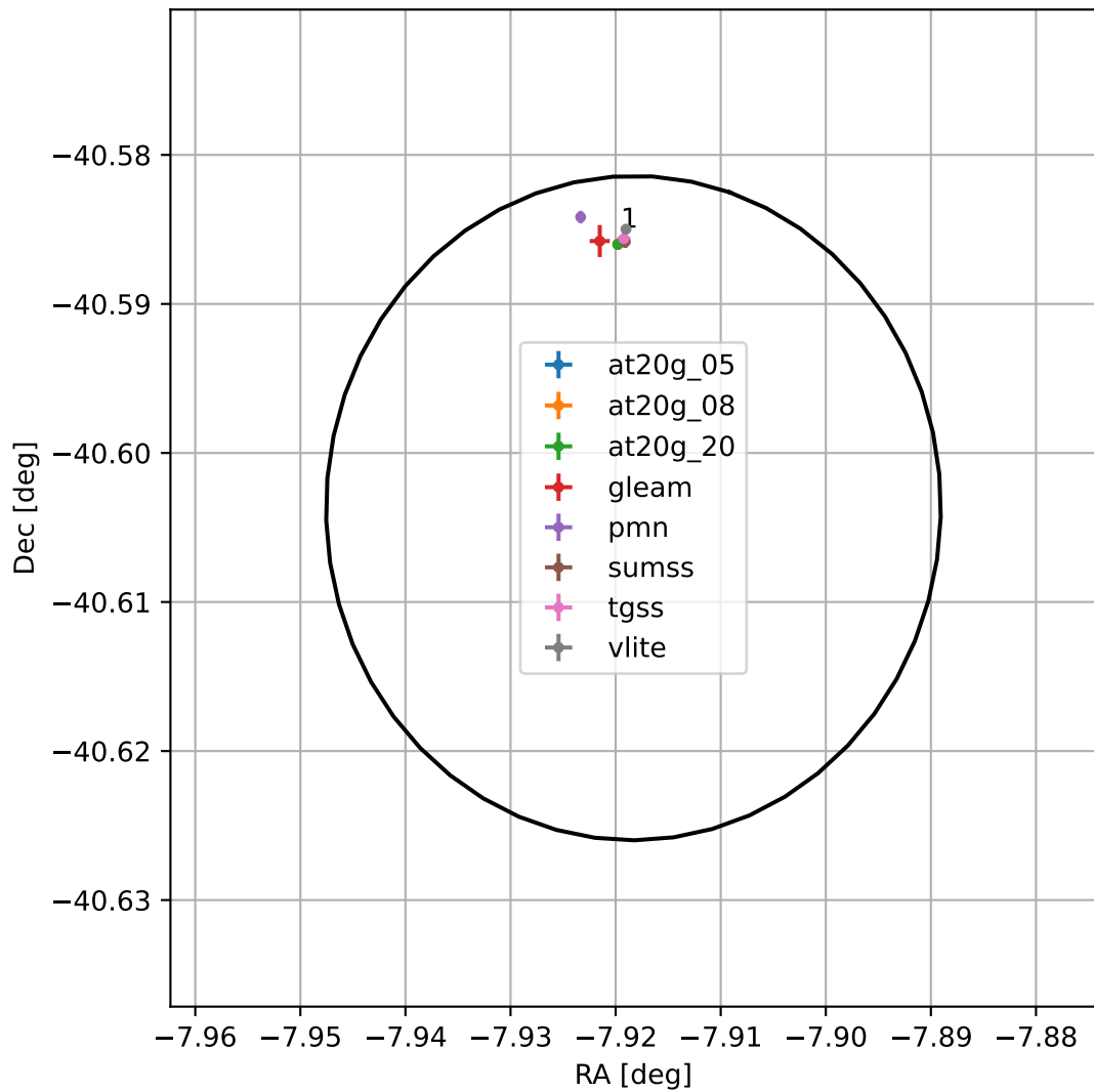
4FGL J2328.3-4036
