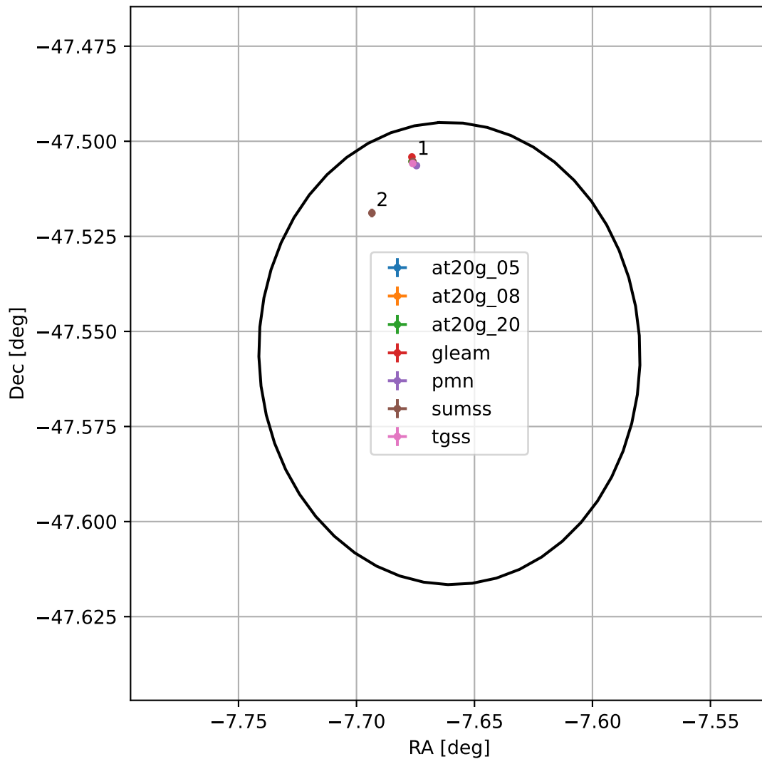
4FGL J2329.3-4733
