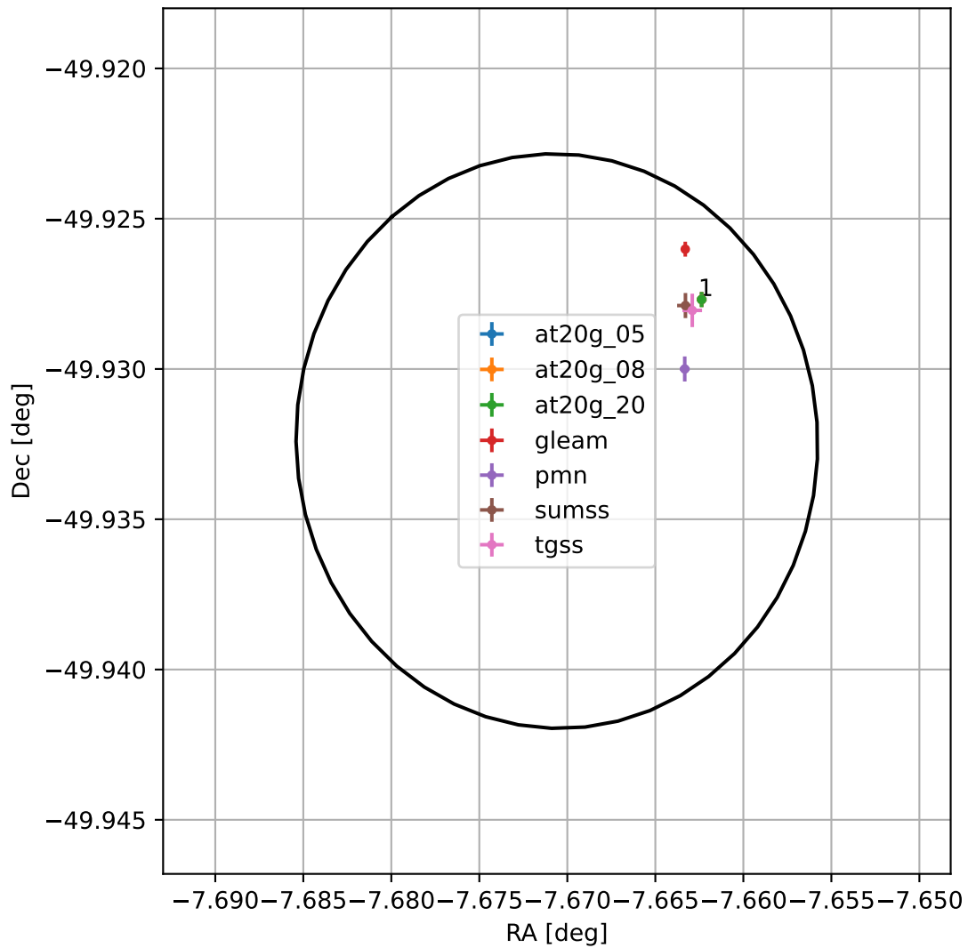
4FGL J2329.3-4955
