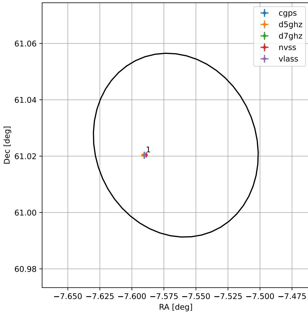
4FGL J2329.7+6101
