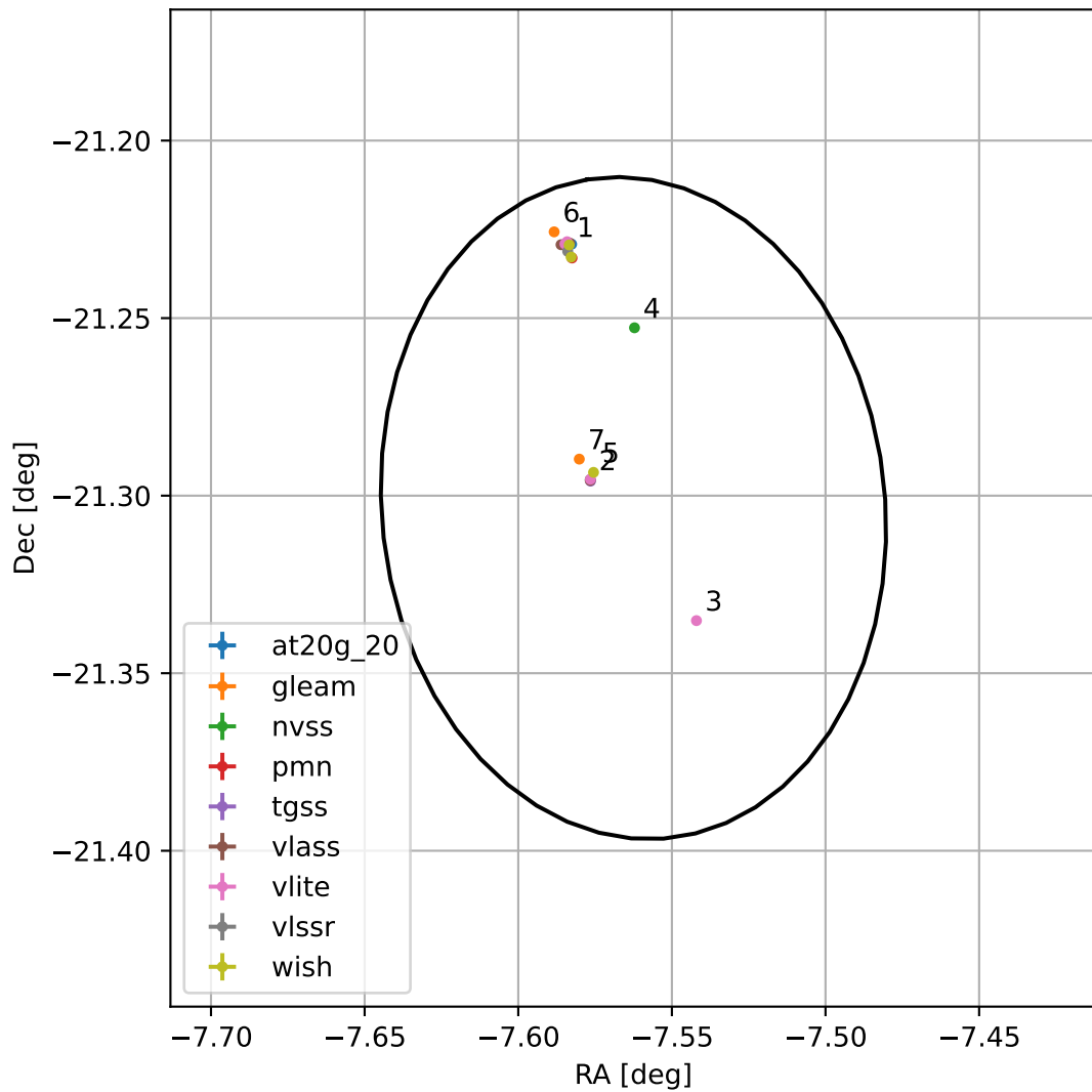
4FGL J2329.7-2118
