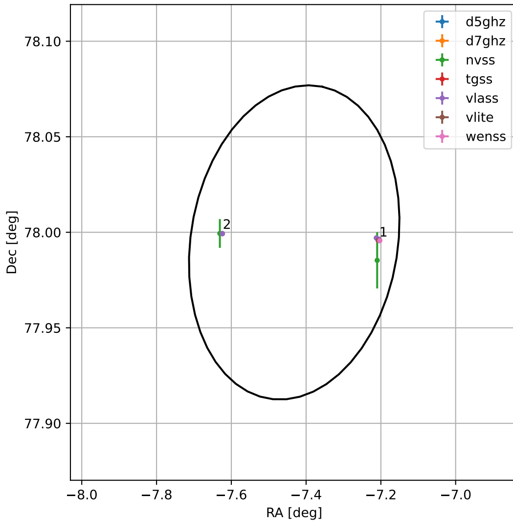
4FGL J2330.2+7759
