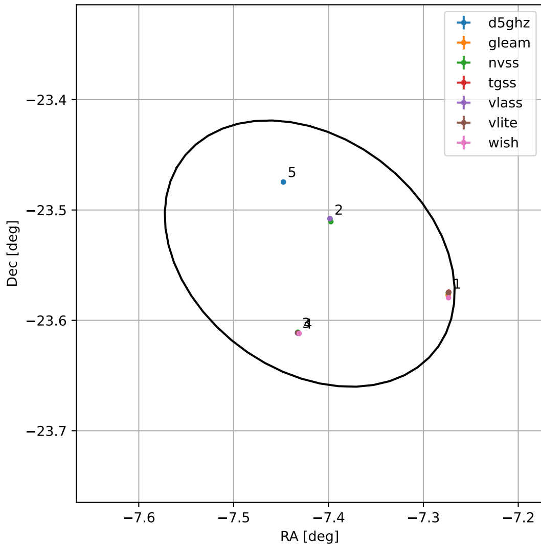
4FGL J2330.3-2332
