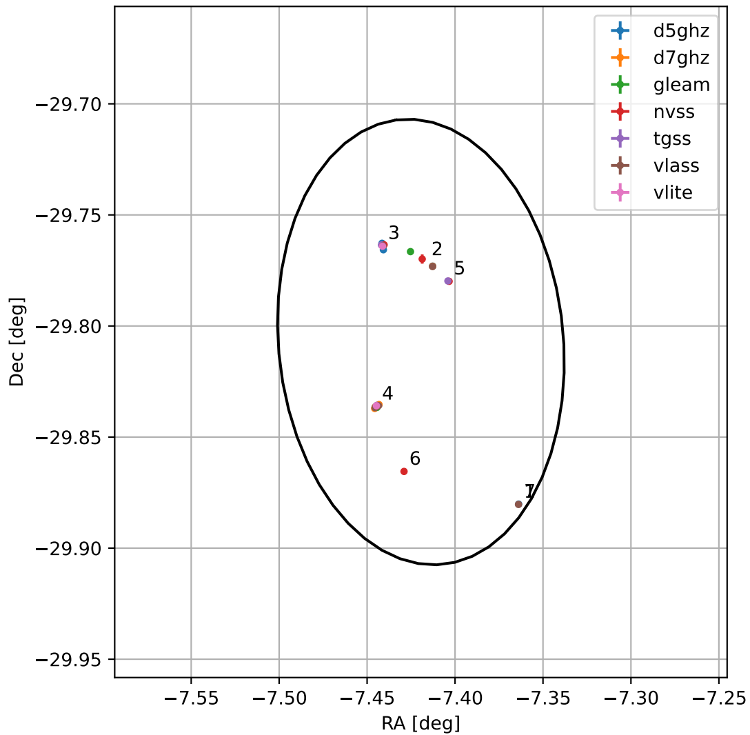
4FGL J2330.3-2948
