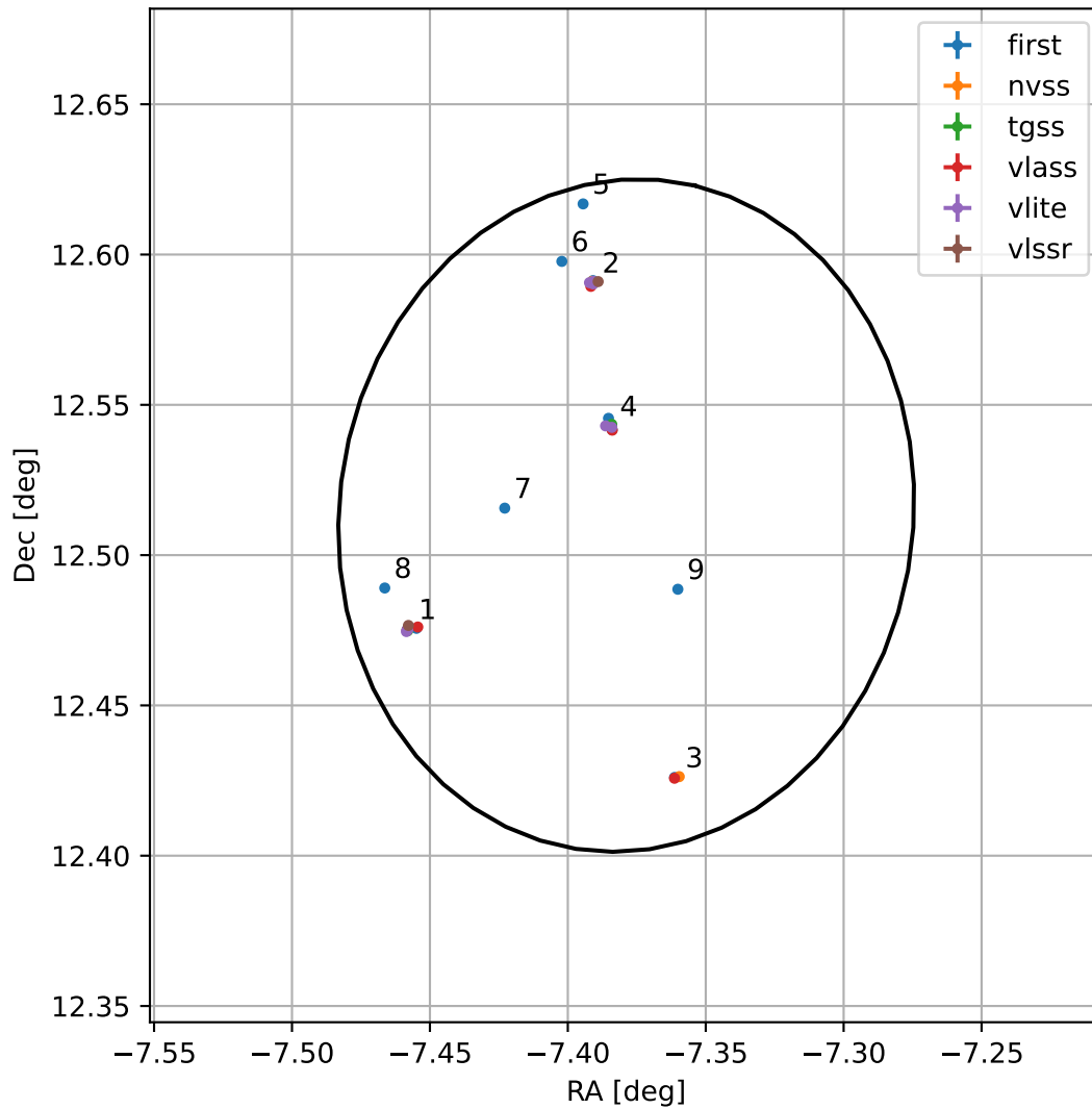
4FGL J2330.4+1230
