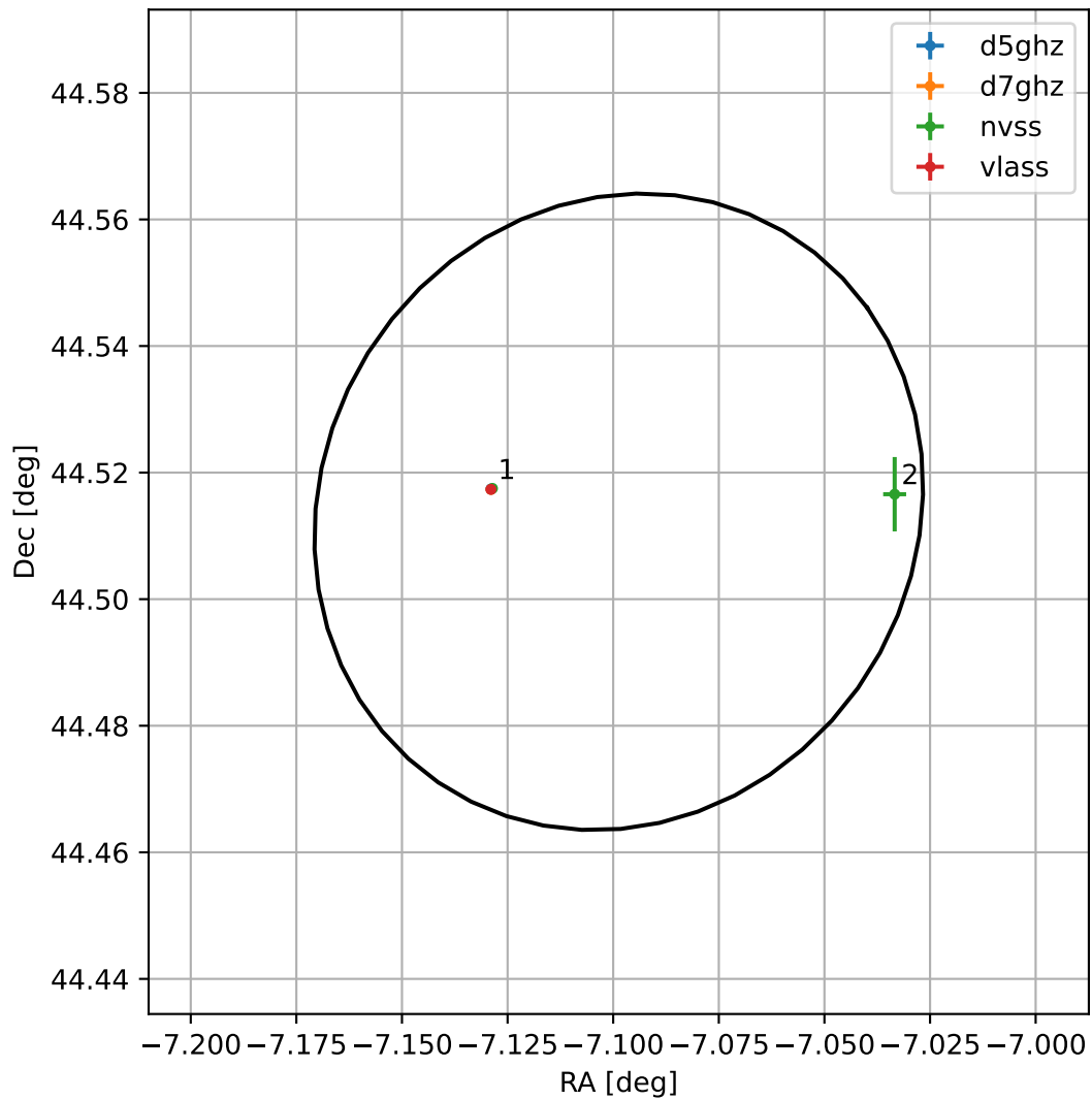
4FGL J2331.6+4430
