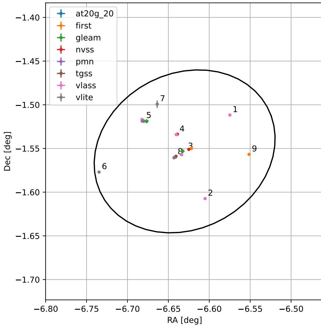
4FGL J2333.4-0133
