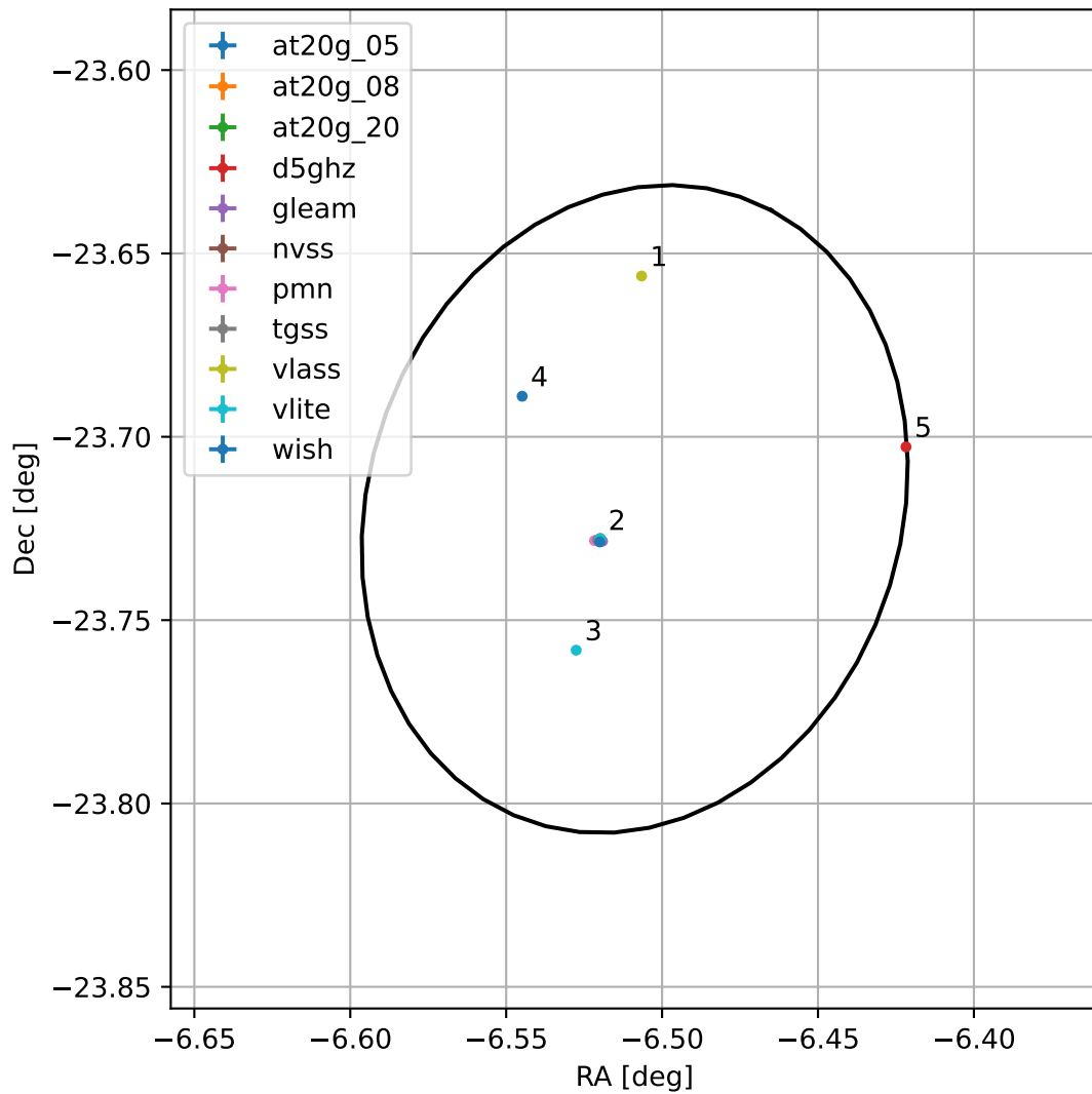
4FGL J2333.9-2343
