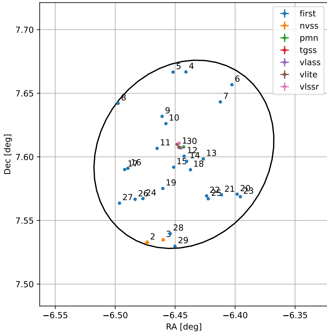
4FGL J2334.2+0736
