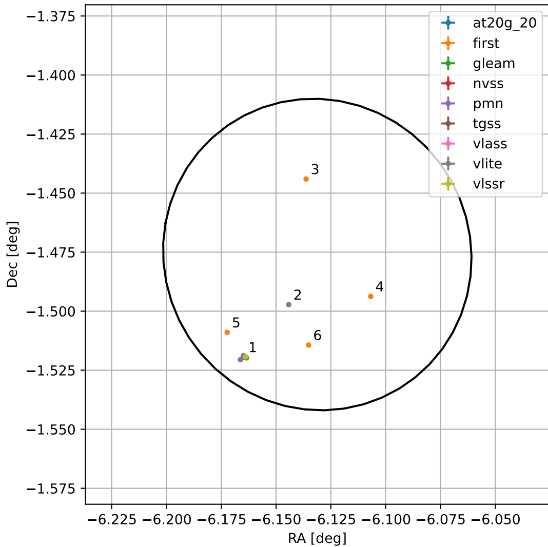
4FGL J2335.4-0128
