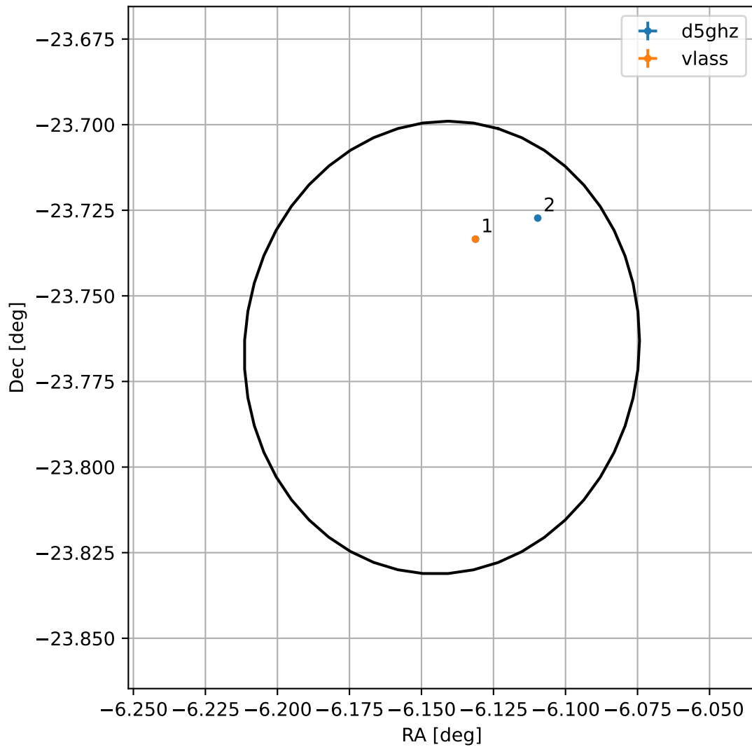
4FGL J2335.4-2345
