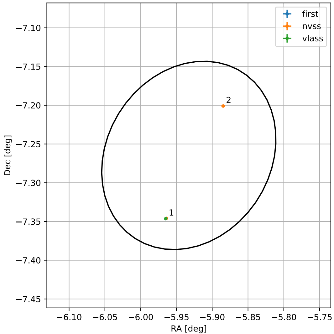
4FGL J2336.2-0715
