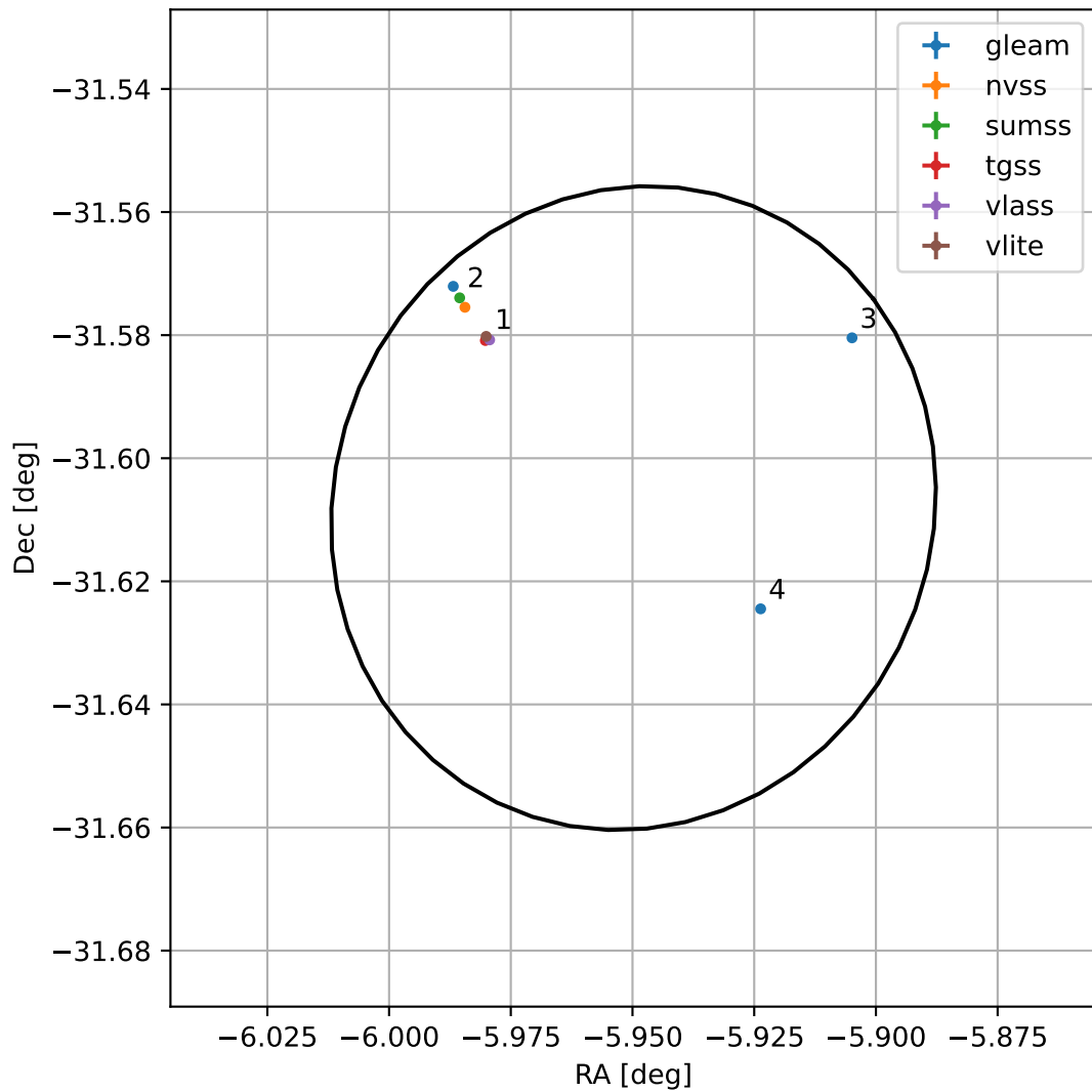
4FGL J2336.2-3136
