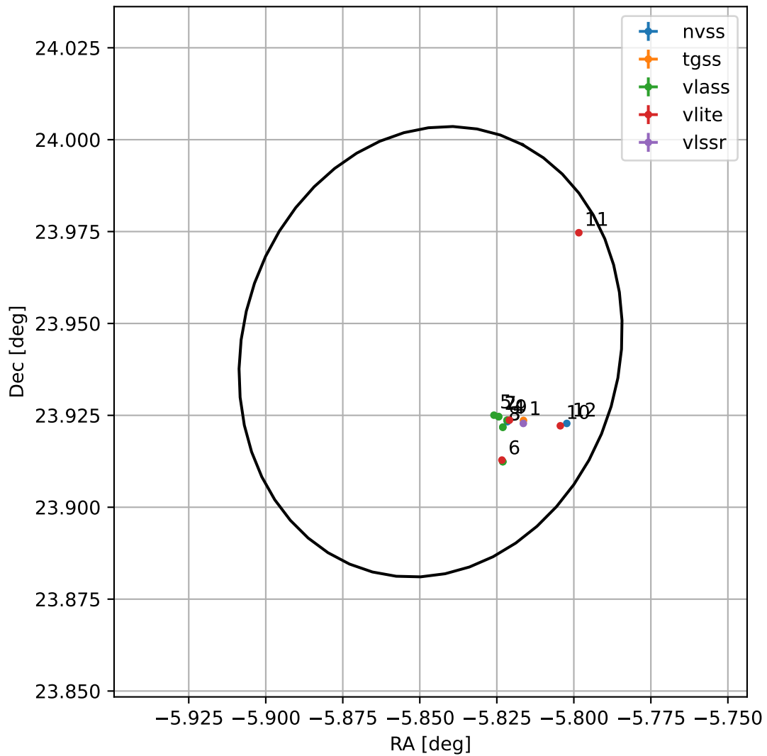
4FGL J2336.6+2356
