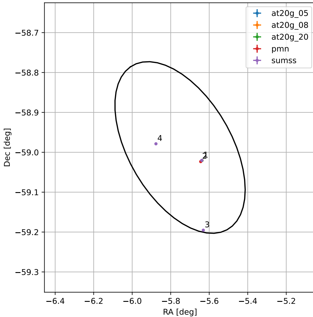
4FGL J2336.9-5859
