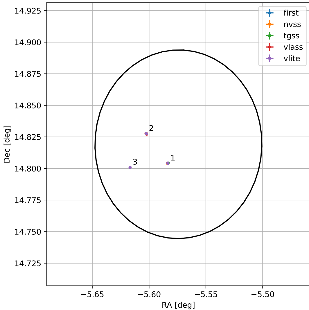
4FGL J2337.7+1449
