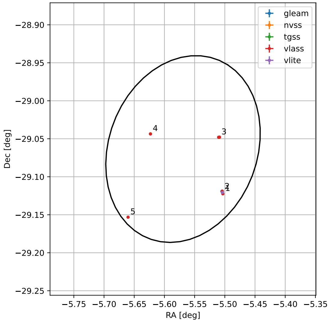
4FGL J2337.7-2903
