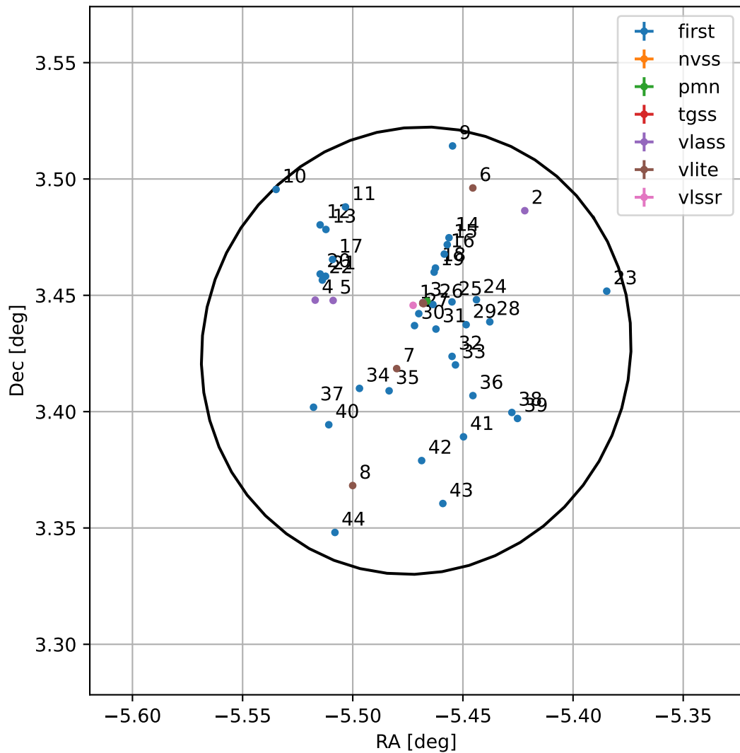
4FGL J2338.1+0325
