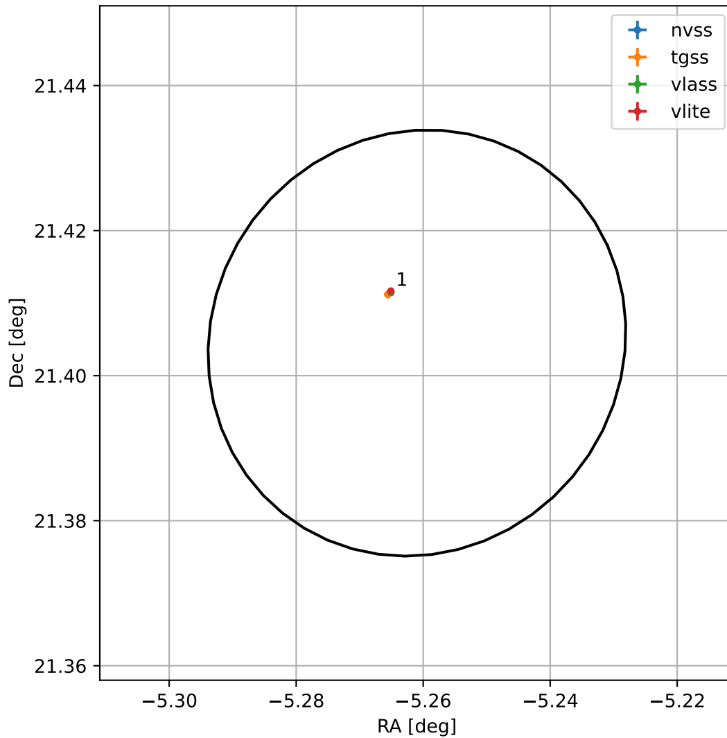
4FGL J2338.9+2124
