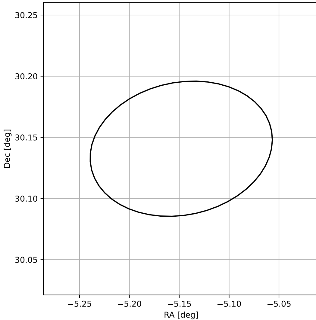
4FGL J2339.4+3008
