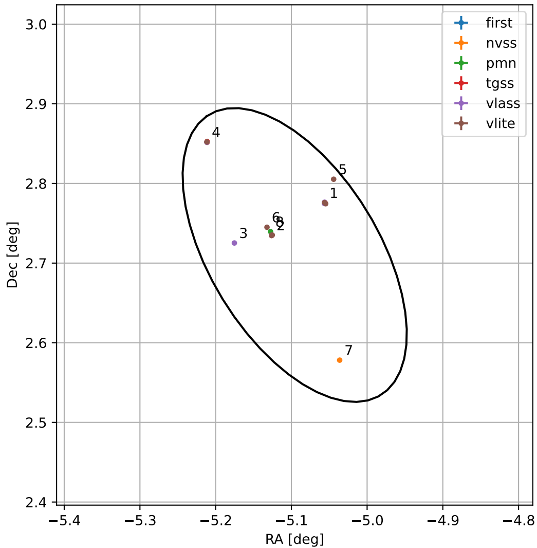
4FGL J2339.6+0242
