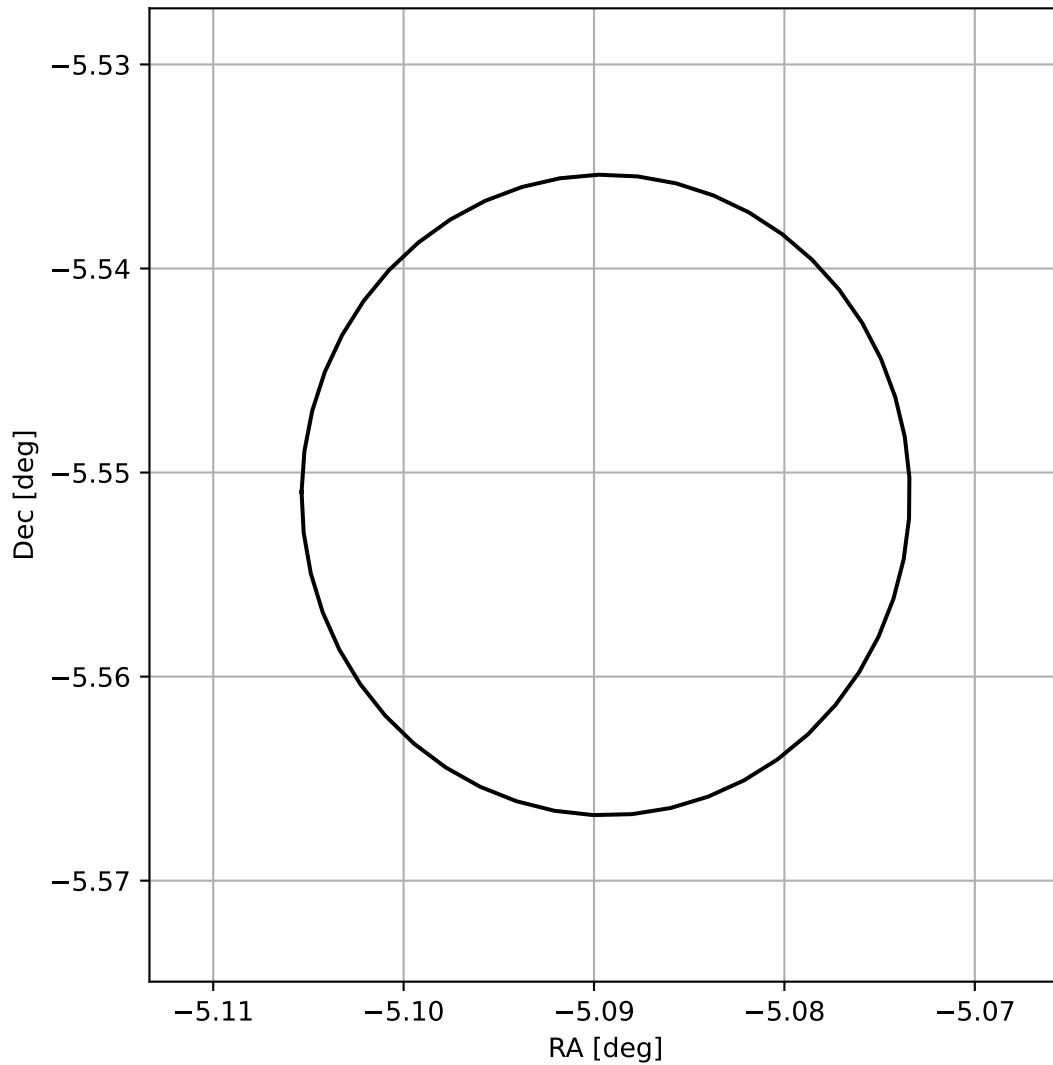
4FGL J2339.6-0533
