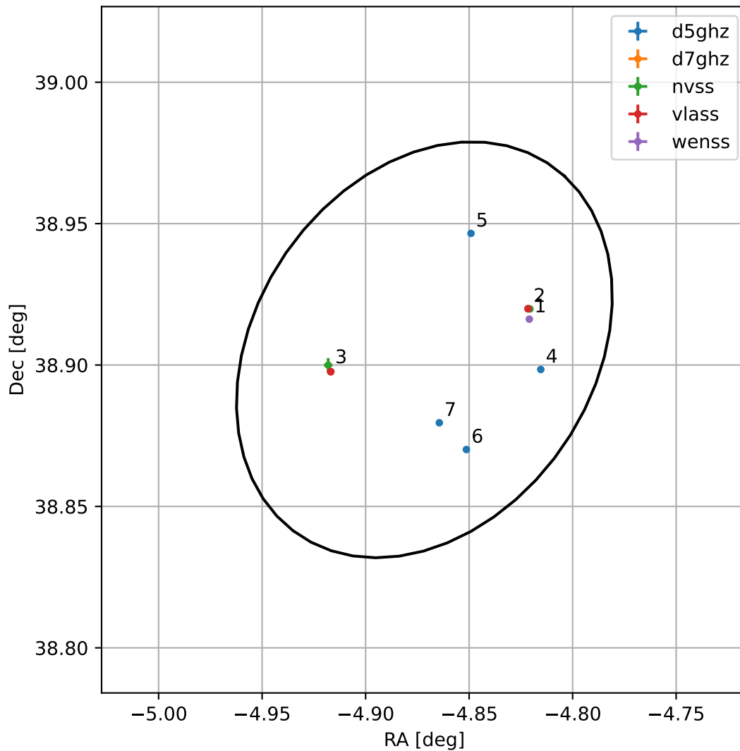
4FGL J2340.5+3854
