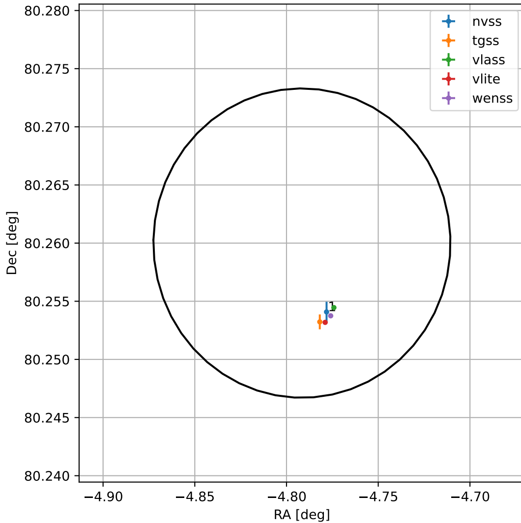
4FGL J2340.8+8015
