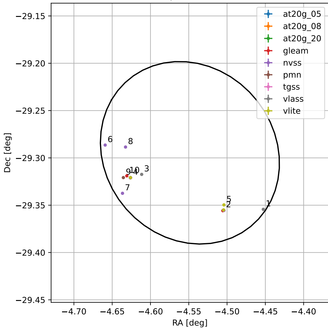
4FGL J2341.8-2917
