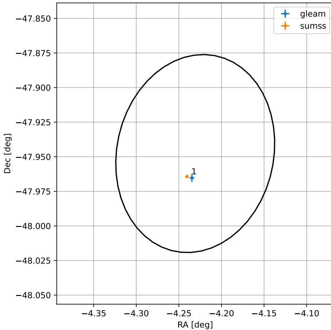
4FGL J2343.0-4756
