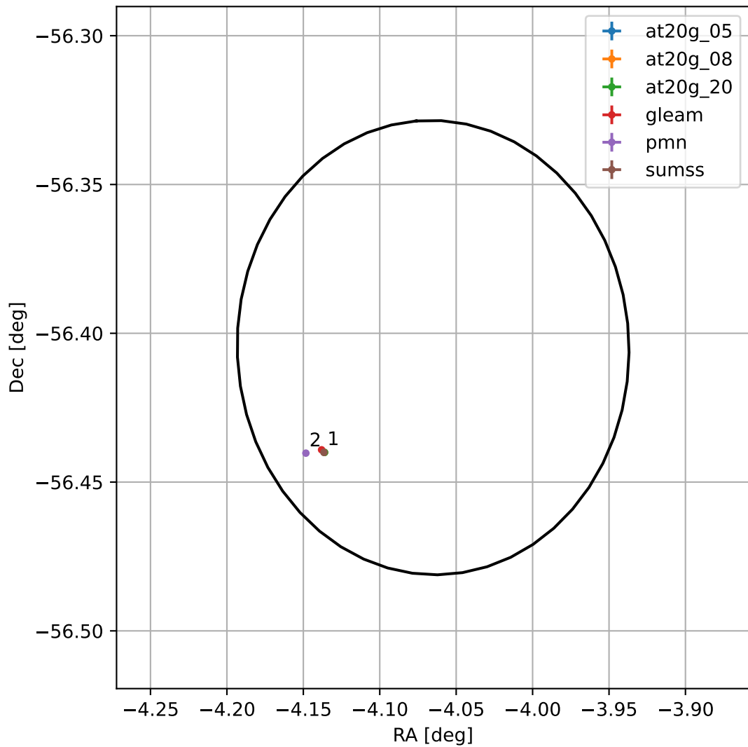
4FGL J2343.7-5624
