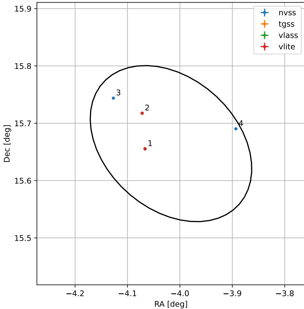
4FGL J2343.9+1539
