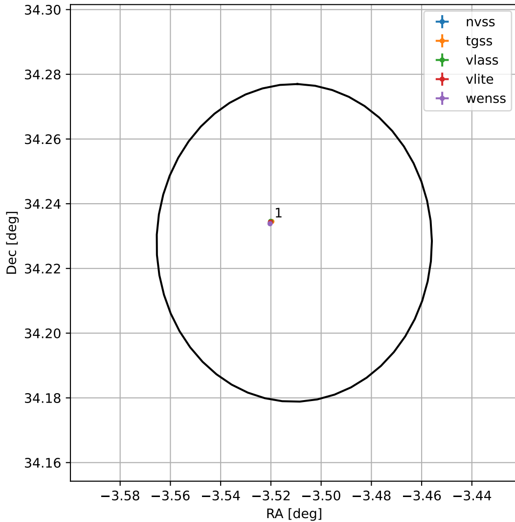
4FGL J2345.9+3413
