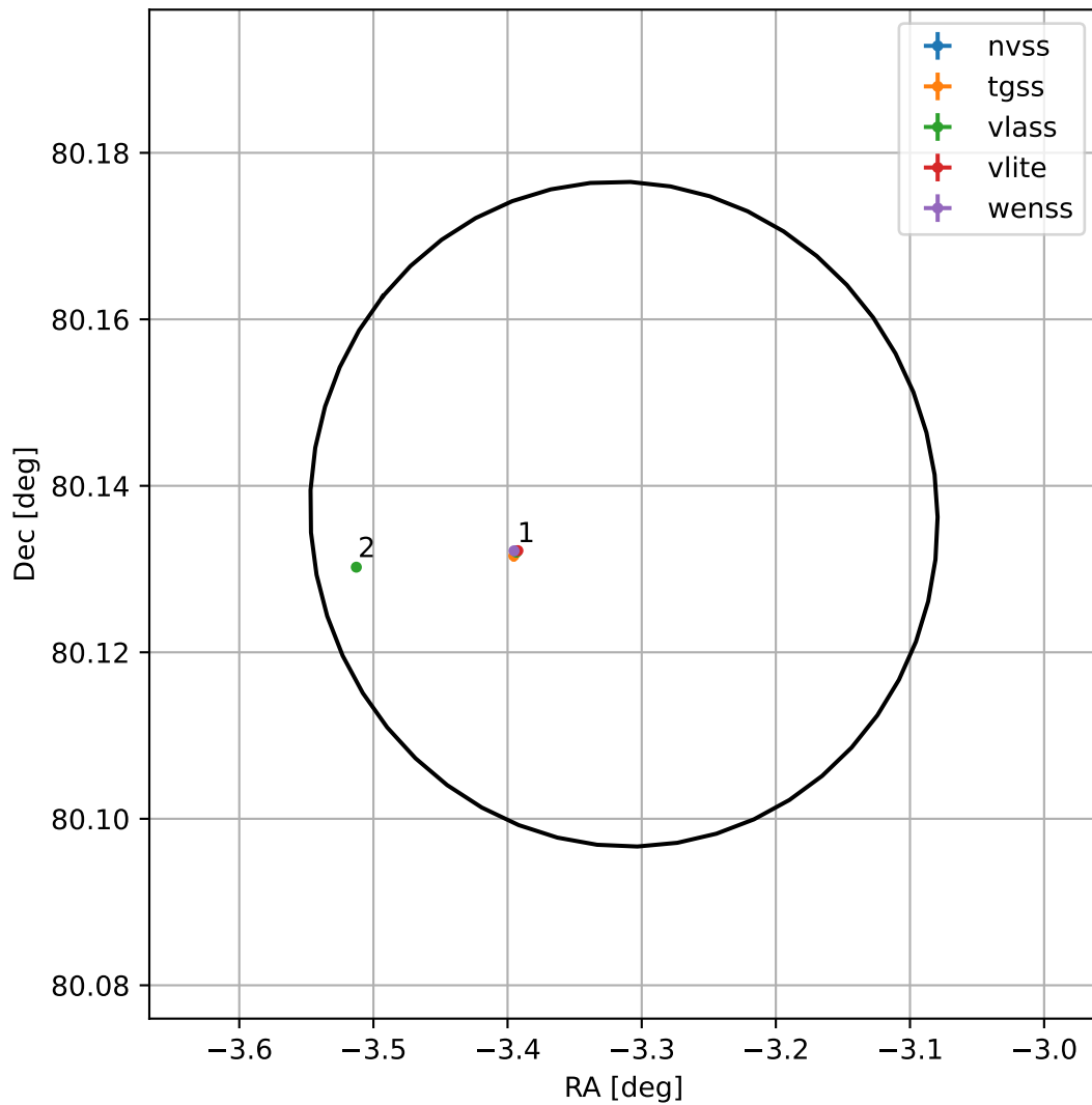
4FGL J2346.7+8008
