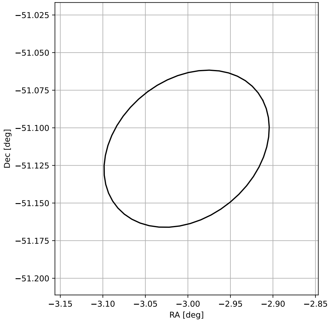
4FGL J2347.9-5106
