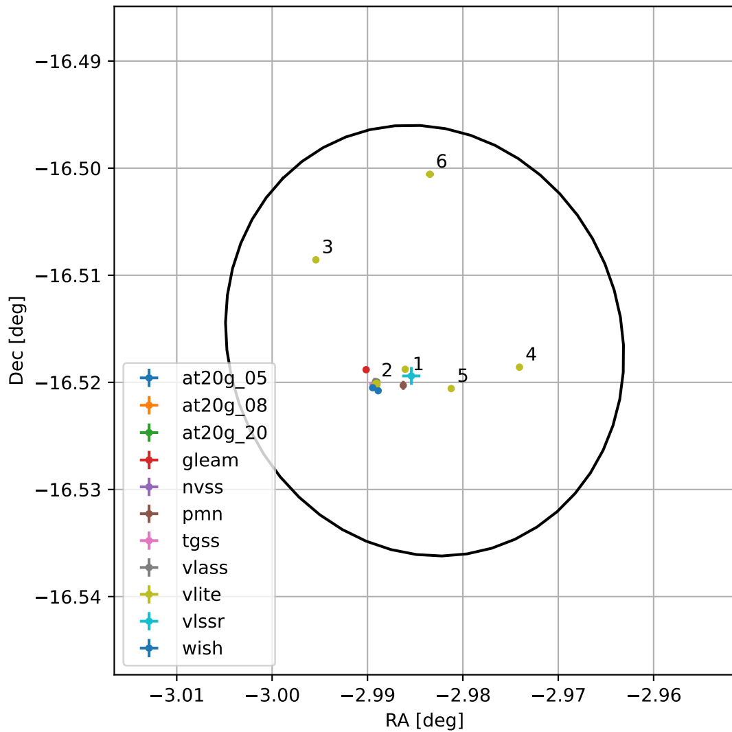
4FGL J2348.0-1630
