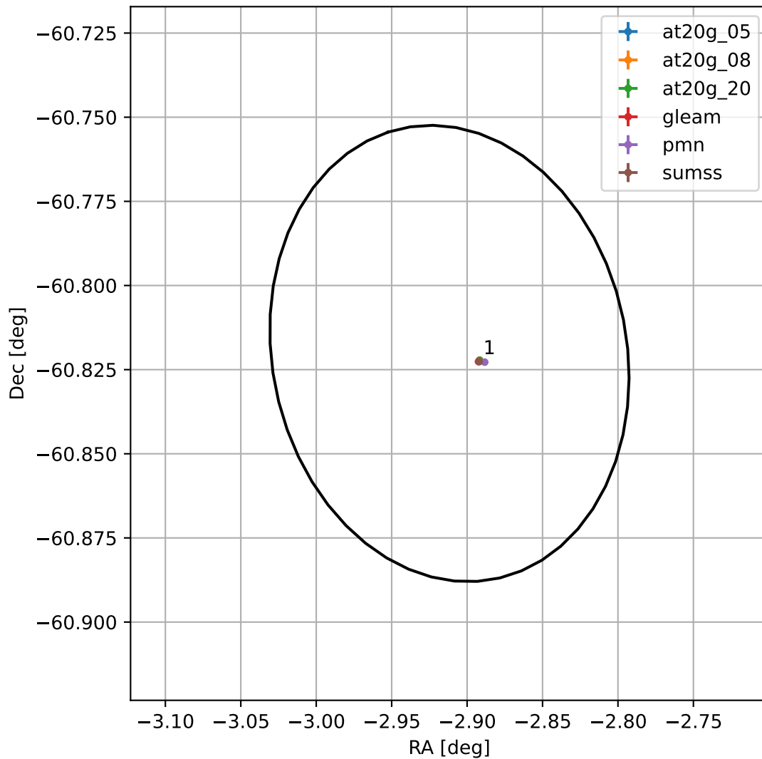
4FGL J2348.3-6049
