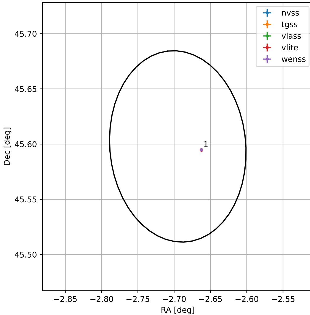
4FGL J2349.2+4535
