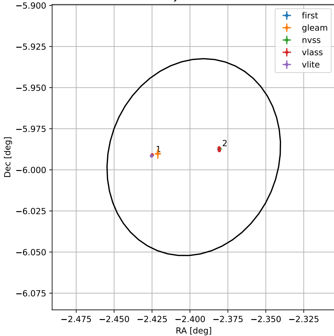
4FGL J2350.4-0559
