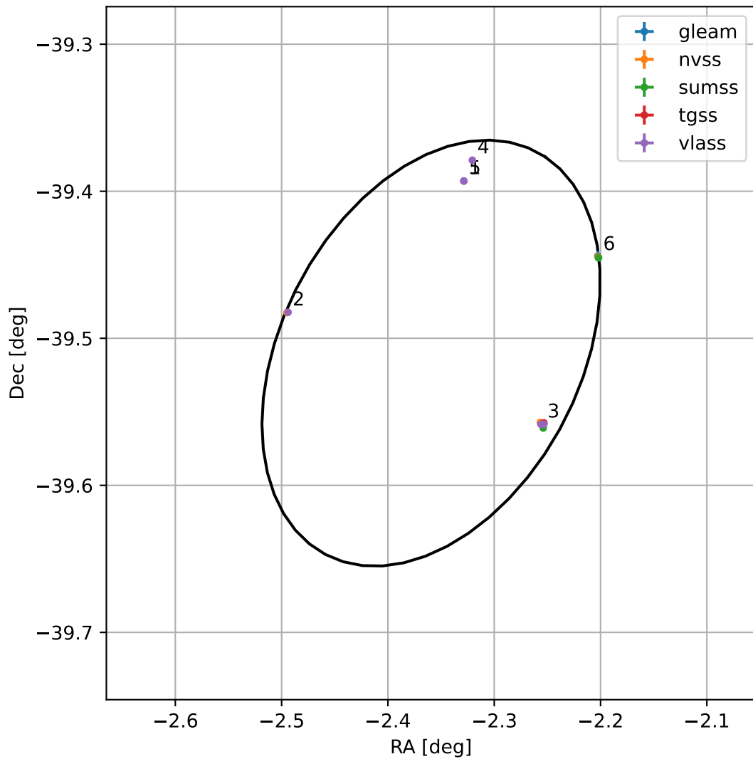
4FGL J2350.5-3930
